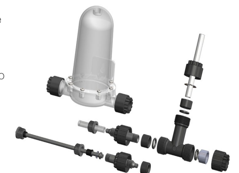
Exploded View of Large Bore Fittings Range
