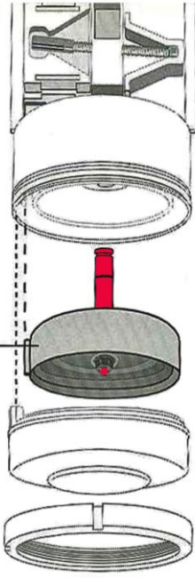
DIAPHRAGM ASSEMBLY ATS/443 (WITH PRE-GREASED SHAFT)
