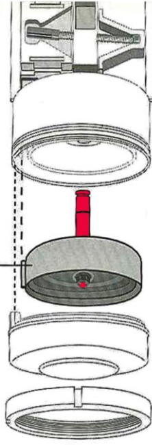
DIAPHRAGM ASSEMBLY ATS/443 (WITH PRE-GREASED SHAFT)
